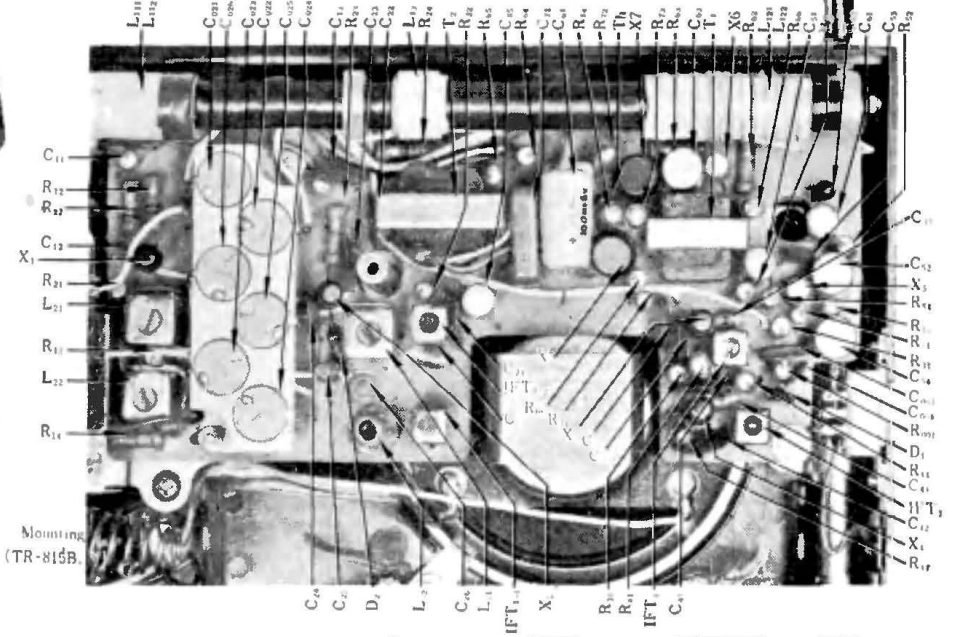
TR-815B and TR-815Y Mounted circuit board
