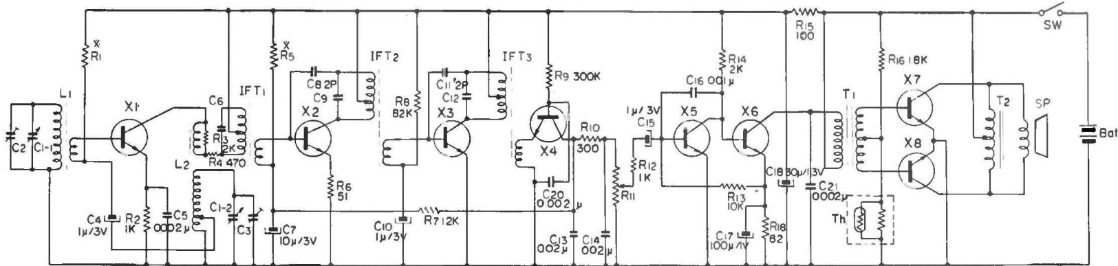
Schematic Diagram
